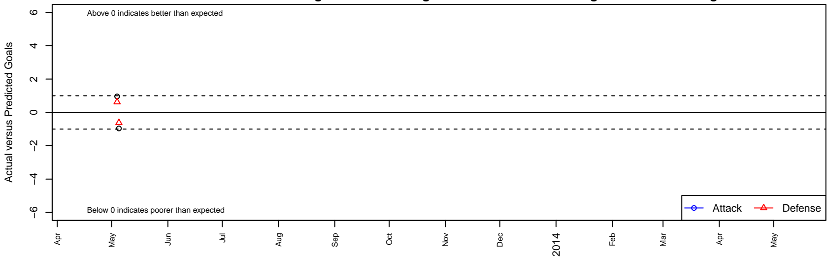
Legacy FC Maroon B99 Dots are actual minus expected GF (blue circles) and GA (red triangles). Blue line is smoothed change in attack strength. Red is smoothed change in defense strength.
